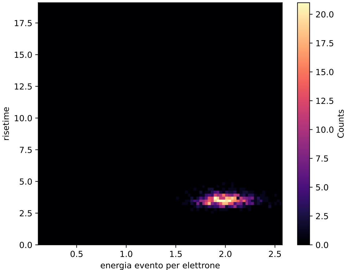
electron distribution 2.0GeV
