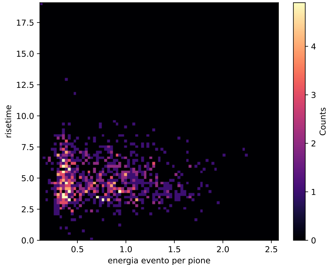
pion distribution 2.0GeV
